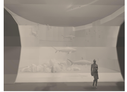
Tank Dim. - 90' L x 49' 8" W x 25' H
